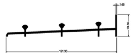
8025-12 UMBRAL 2 VIAS BRONCE 5.8 MTS
