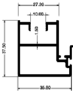
8025-7 VERTICAL CENTRO BRONCE
