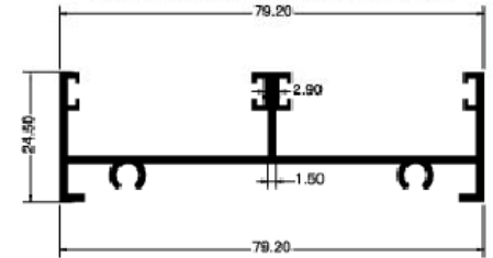
8025-3 JAMBA BRONCE 5.8 MTS
